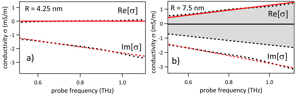
Figure 4.2: Exemplary THz conductivity spectra (black dots) for CdTe nanocrystal samples showing a) no real conductivity and b) finite real conductivity. Red solid (real part) and dashed (imaginary part) lines are the results of models for the exciton polarizability described in the text. The black lines in b) show the electron contribution to the total exciton polarizability for this radius, and the grey-shaded area the hole contribution.
