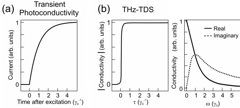
Figure 1.6: Time dependence of signals in a (a) transient photoconductivity measurement and (b) THz-TDS measurement, both for a Drude electron gas undergoing a step increase in density at time zero.
