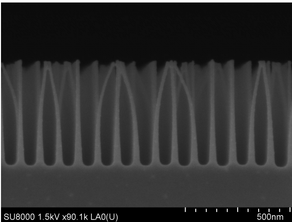
Figure 3.2: Scanning electron microscope image of the nanowires after thermal oxidation. The thermal oxide was removed by vapor HF for this SEM image but not for the terahertz spectroscopy.
